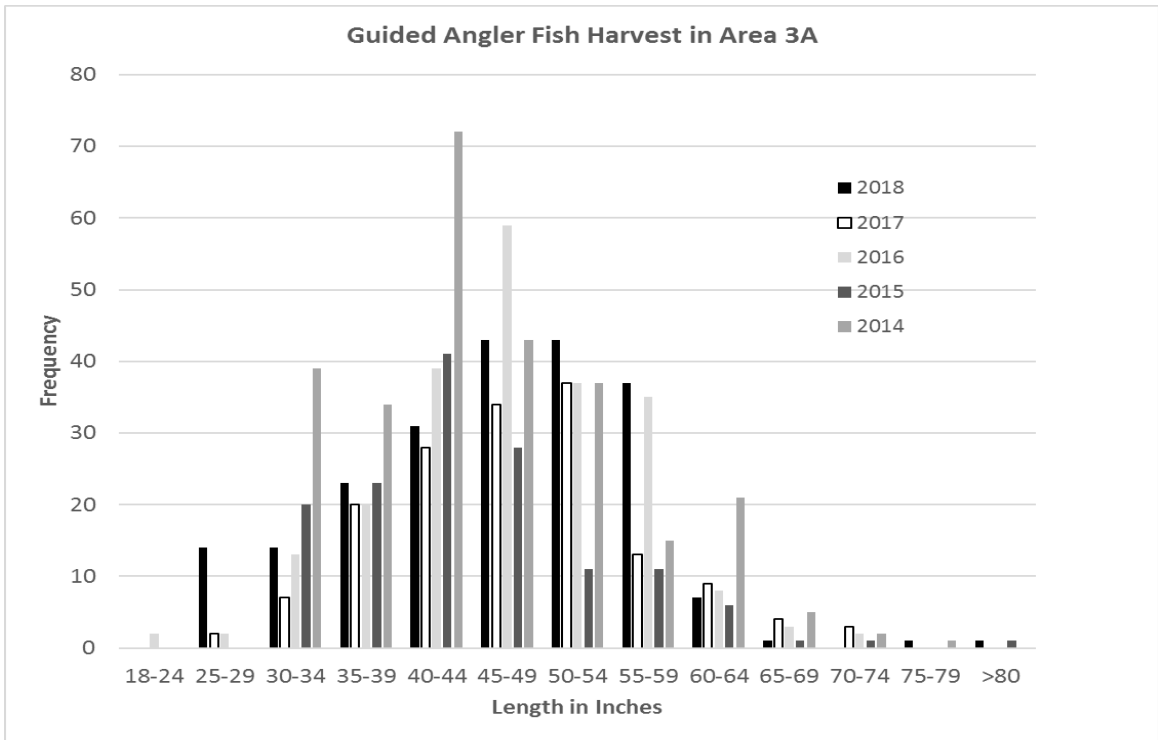
Figure 2. 2014 through 2018 GAF length frequency distribution in IPHC Regulatory Area 3A.
