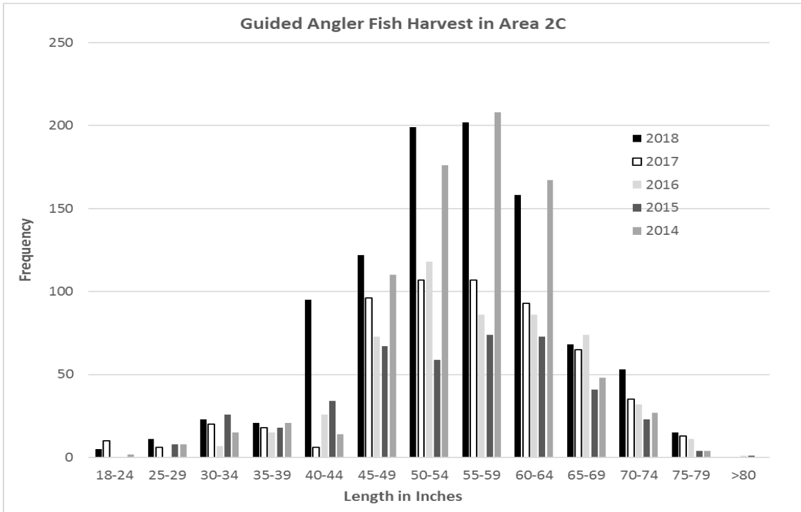
Figure 1. 2014 through 2018 GAF length frequency distribution in IPHC Regulatory Area 2C.
