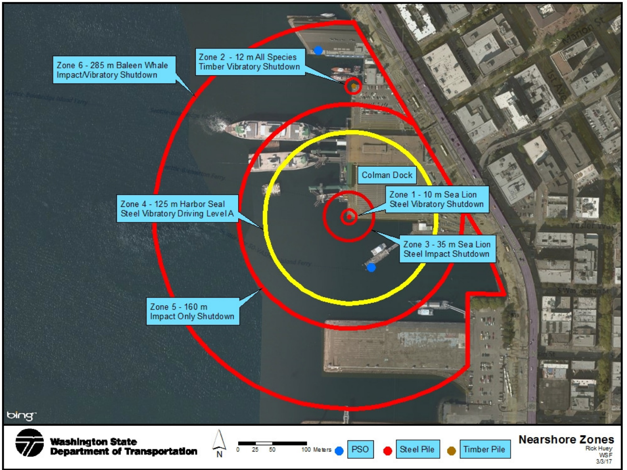
Figure 1 – Nearshore Zones
