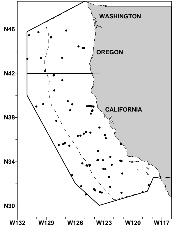
Figure 1. Sperm whale sighting locations based on aerial and shipboard surveys off California, Oregon, and Washington, 1991-2001. Dashed line represents the U.S. EEZ, thick line indicates the outer boundary of all surveys combined. Greater effort was conducted off California (south of 42°N) and in the inshore half of the U.S. EEZ. See Appendix 2 for data sources and information on timing and location of survey effort.
